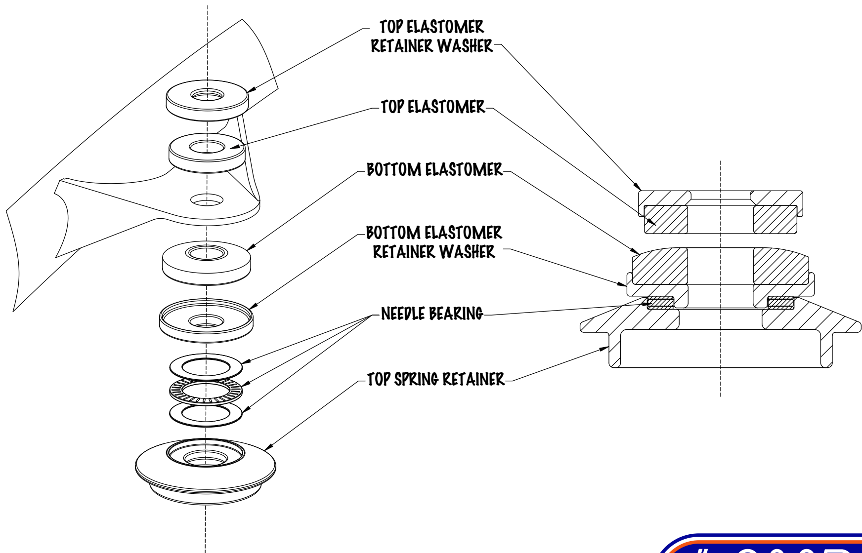
LAMB STRUT TOP MOUNT ASSEMBLY
