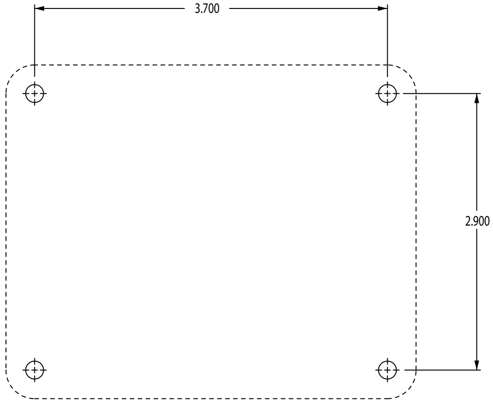
Independent Compression Control Module Mounting Template
